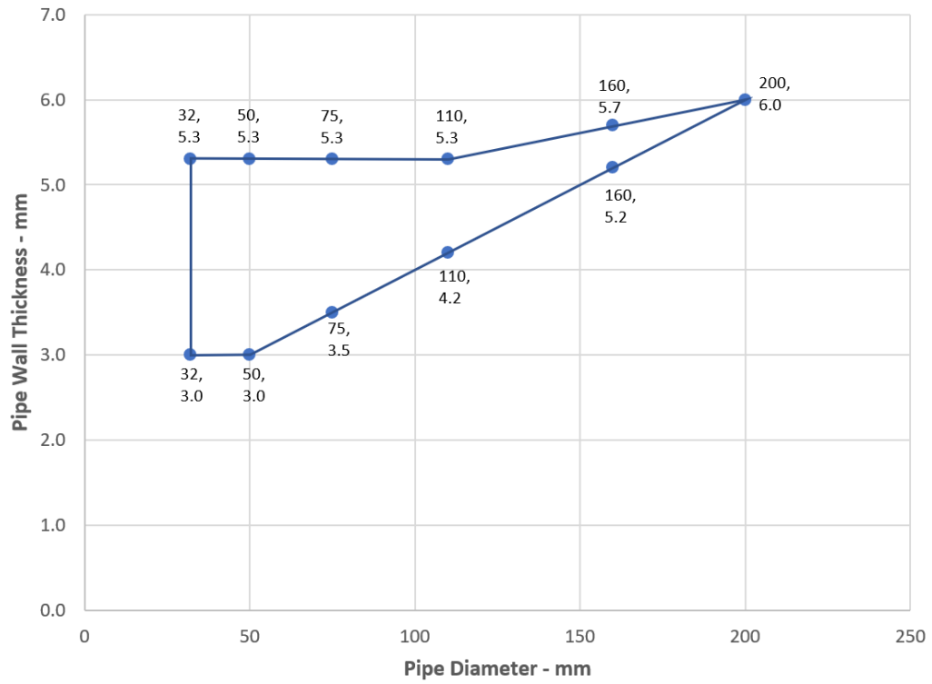
Wavin AS+ Pipes 32-200 / 50 mm Wrap
